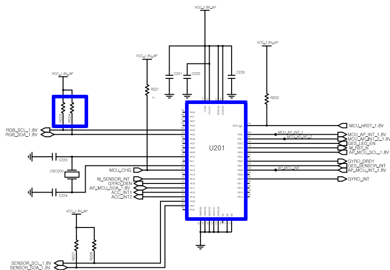
SENSOR HUB
